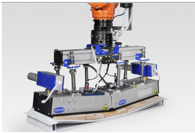
Mounting example flexible suspension FST-FLEX
